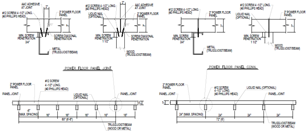
(6'-8" LONG. PANELS - SUPPORTS @ 16" O.C.)
